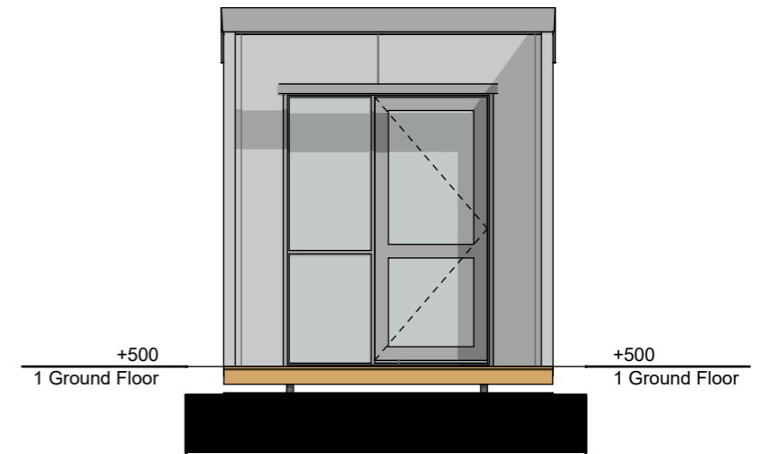
East Elevation
