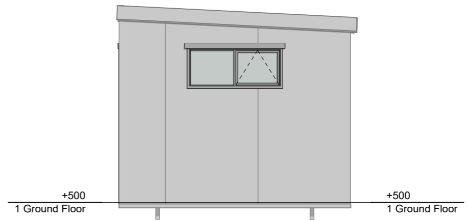
5 West Elevation 1:50
