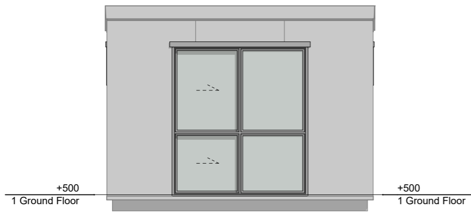
2 North Elevation 1:50
