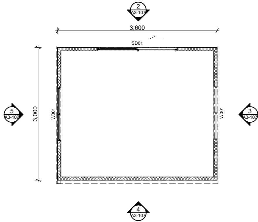
1 Floor Plan 1:50
