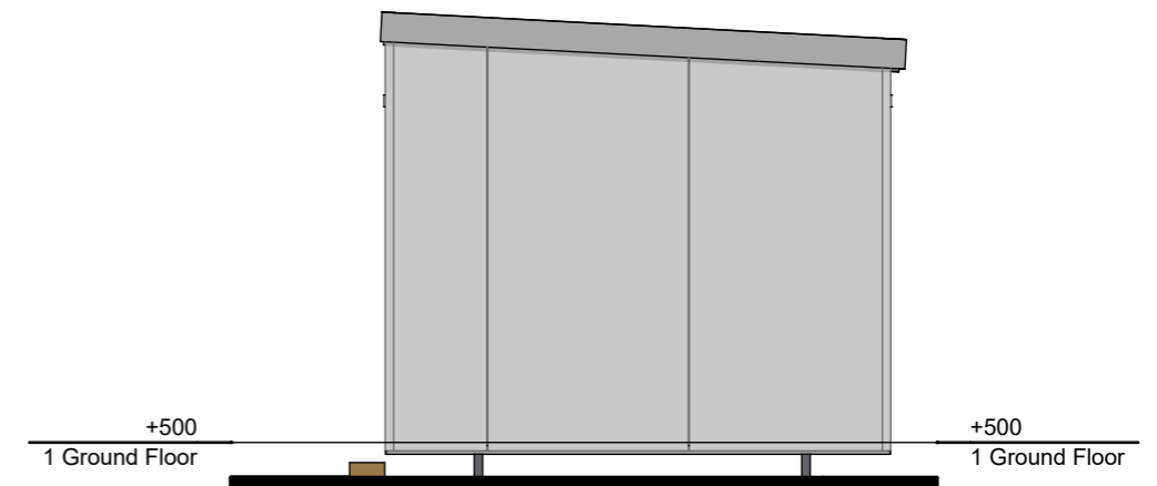
6 West Elevation
