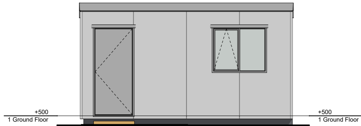
3 North Elevation
