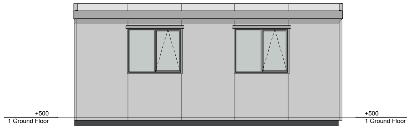
South Elevation
