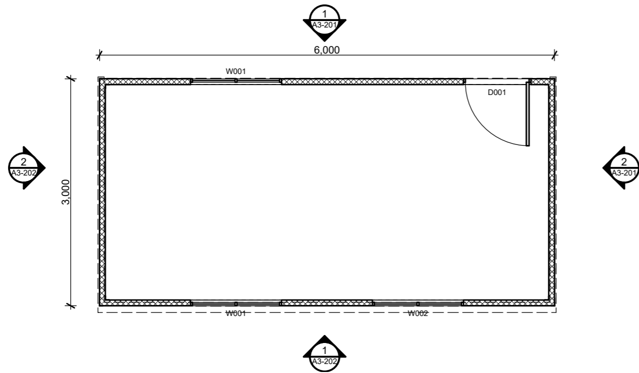
1 Floor Plan
