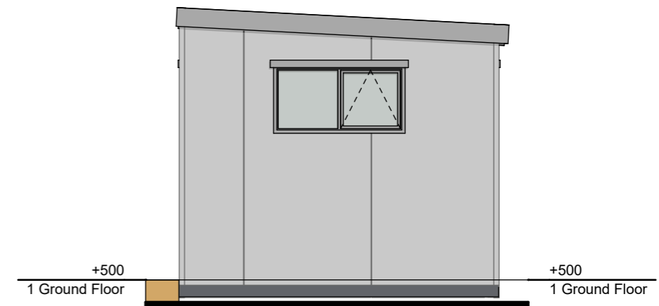
6 West Elevation
