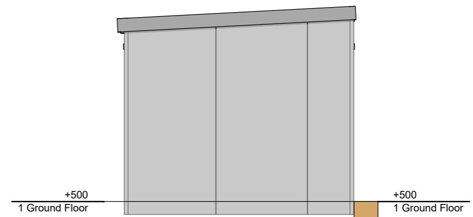
4 East Elevation
