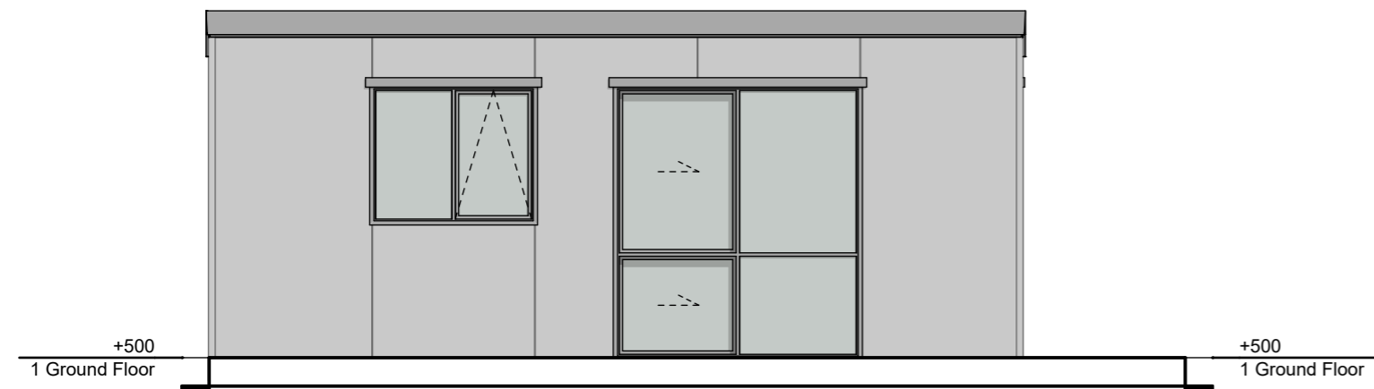
3 North Elevation
