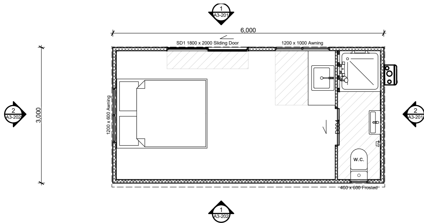
1 Floor Plan
