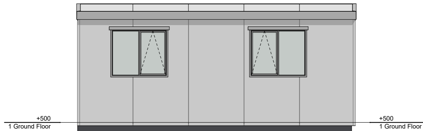
5 South Elevation 1:50
