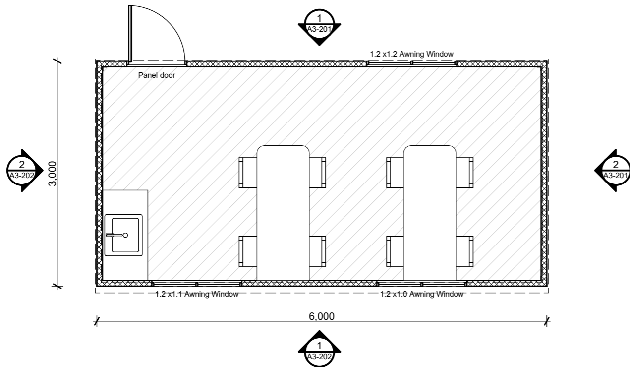
1 Floor Plan 1:50
