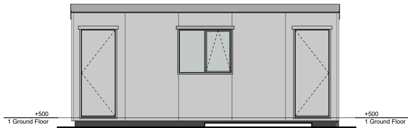
3 North Elevation 1:50
