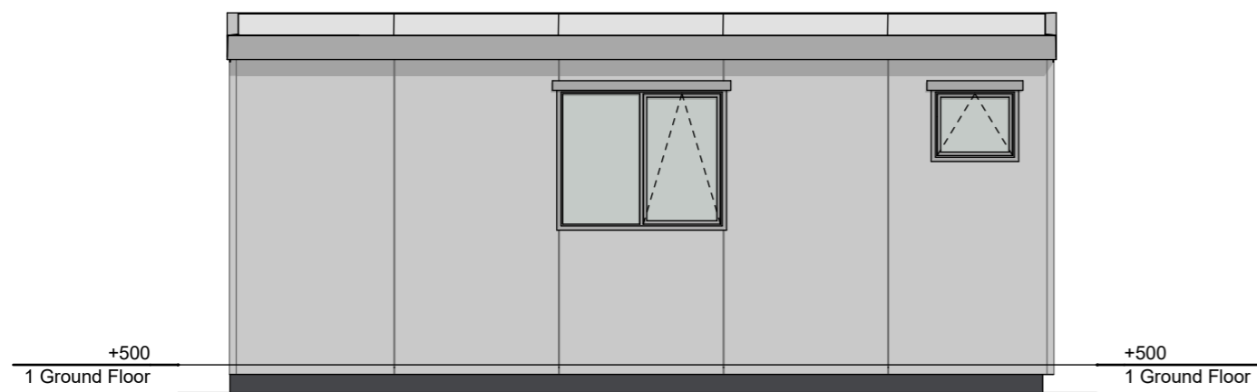
5 South Elevation 1:50
