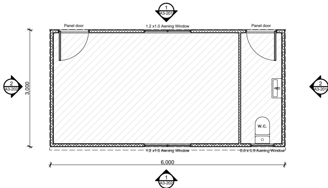
1 Floor Plan 1:50
