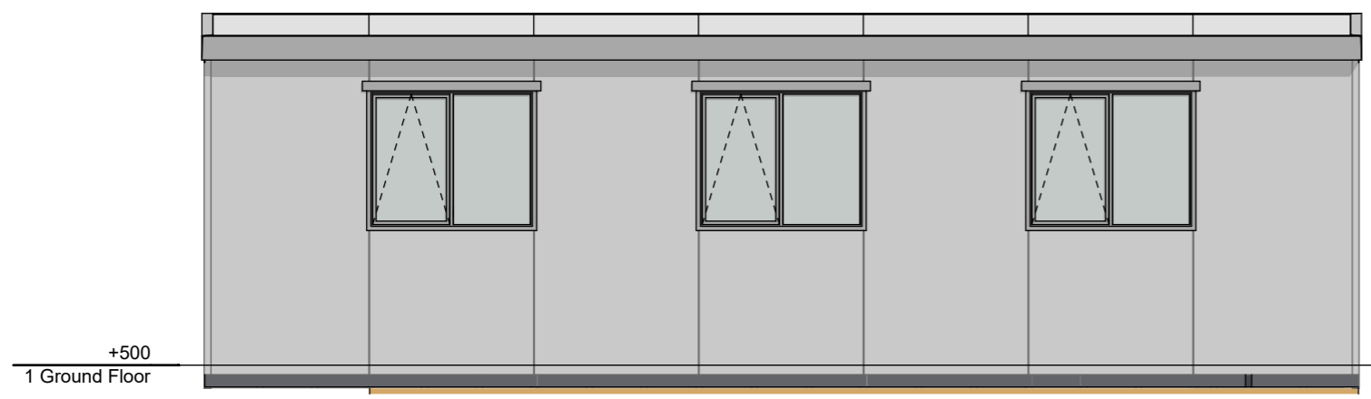
5 South Elevation
