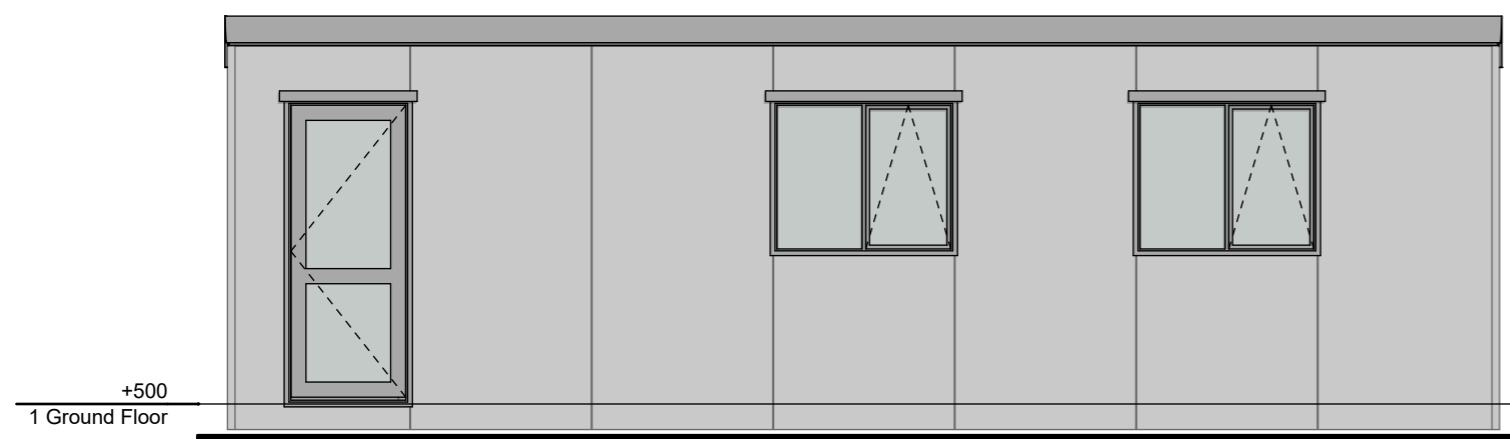
3 North Elevation
